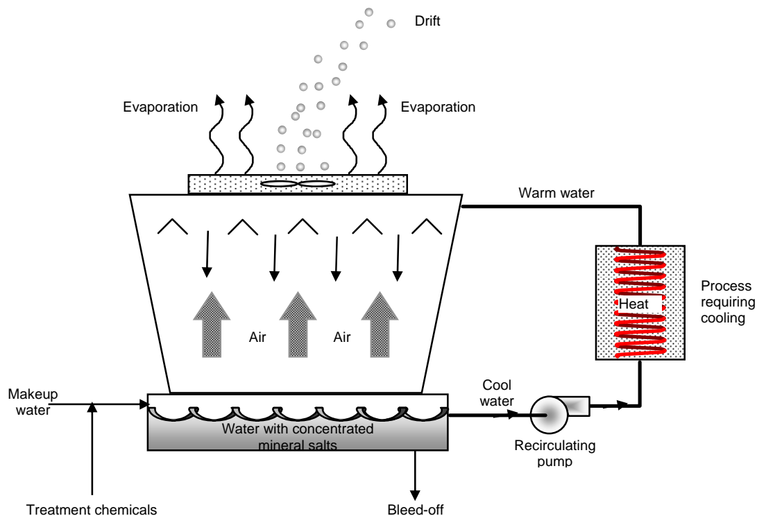
Figure III-1 Cooling Tower Schematic
