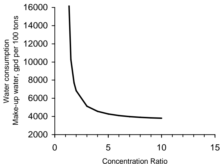
Figure III-2 Cooling Tower Water Consumption vs. Concentration Ratio
