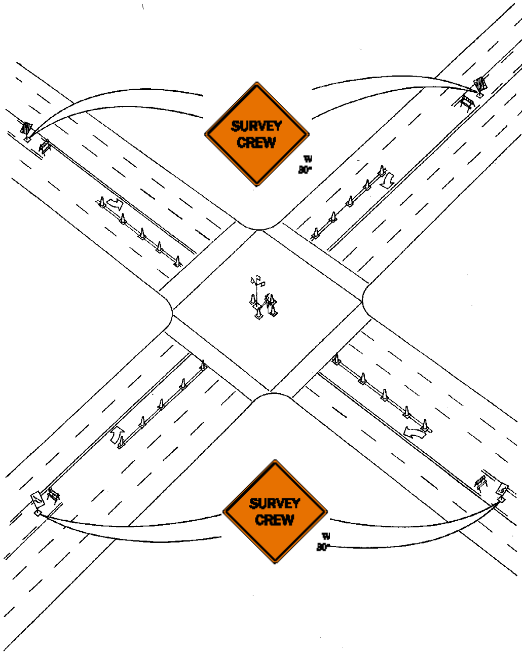
Figure 7-J Surveying Intersection
