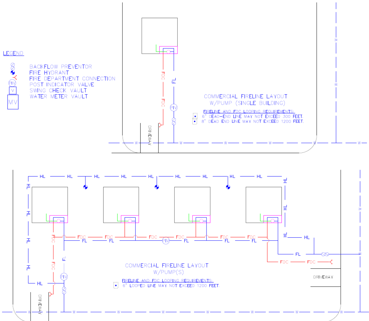
Figure 1-C Commercial Fireline Layout with Pumps
